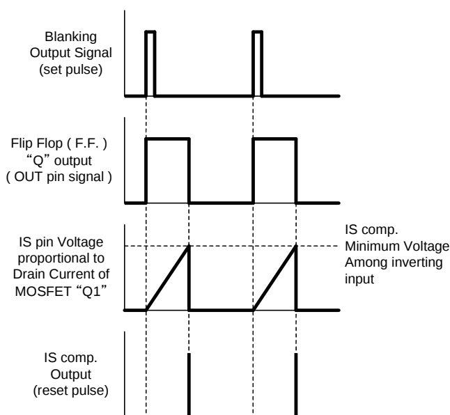
Fig. 6 Timing chart for current-mode basic operation
