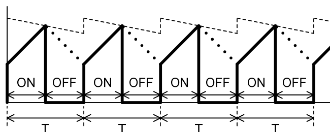
Fig.44 Inductor current with slope compensation
