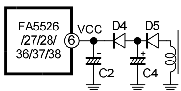
Fig.28 Vcc circuit
