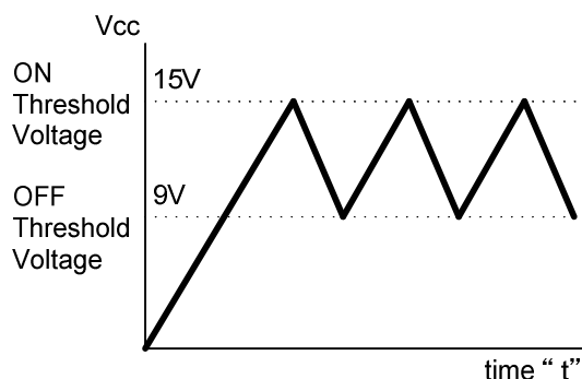
Fig.25 Vcc waveform at start-up (2)
