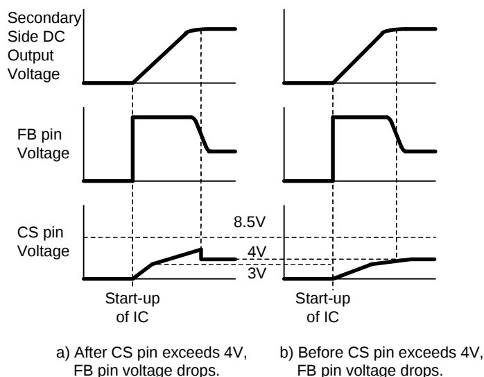
Fig.22 CS pin voltage waveform at start-up (1) ( normal start )
