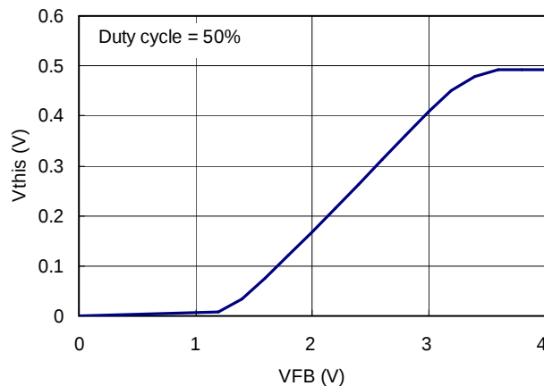
IS pin input threshold voltage (Vth) vs. FB pin voltage (VFB)
