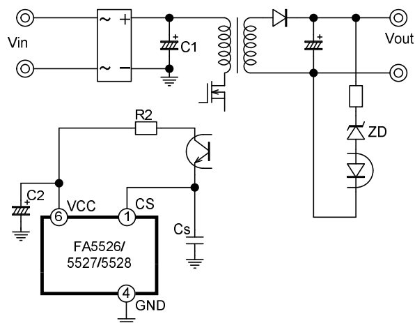
Fig.29 Over Voltage protection (1) for FA5526/27/28
