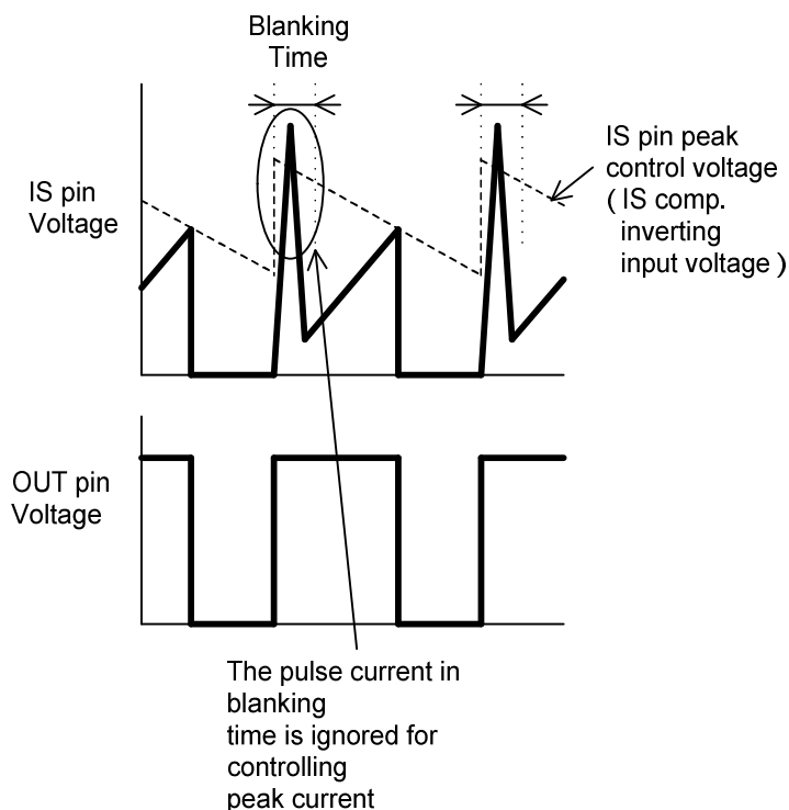
Fig.8 Blanking
