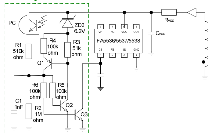
Fig.33 Over Voltage protection (2) for FA5536/37/38
