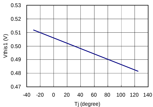
IS pin maximum input threshold voltage (Vth1) vs. Junction Temperature (Tj)
