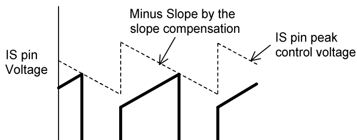
Fig.10 Slope compensation
