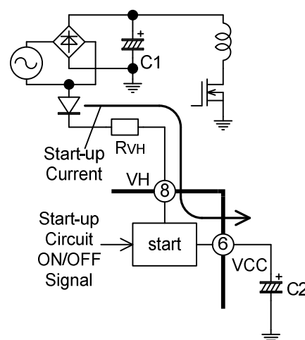
Fig.1 Start-up circuit 1 (half wave)
