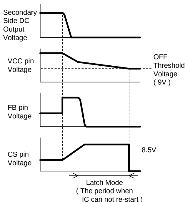
Fig.27 Waveform at stopping (2)
