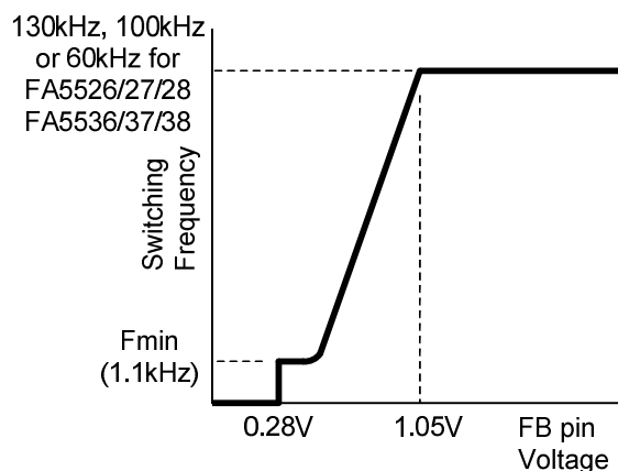
Fig.4 Oscillating frequency
