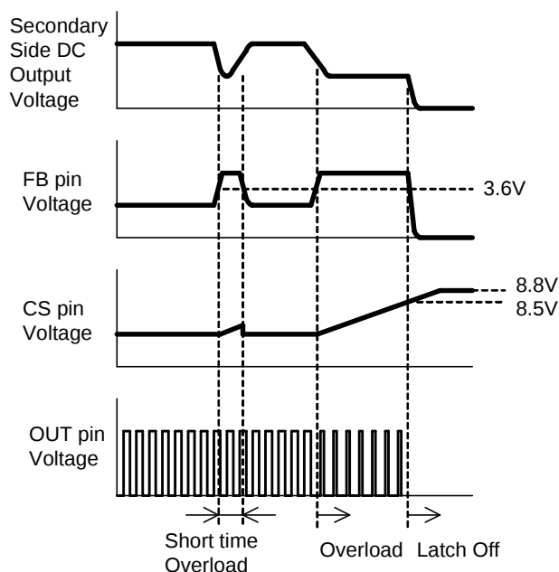
Fig.13 Overload protection timing chart
