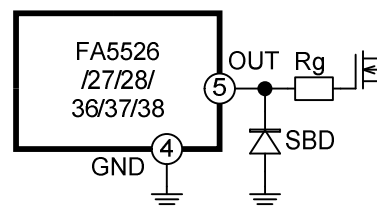
Fig.40 Negative voltage prevention circuit
