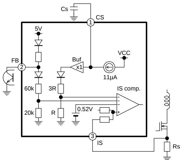
Fig.7 Current comparator
