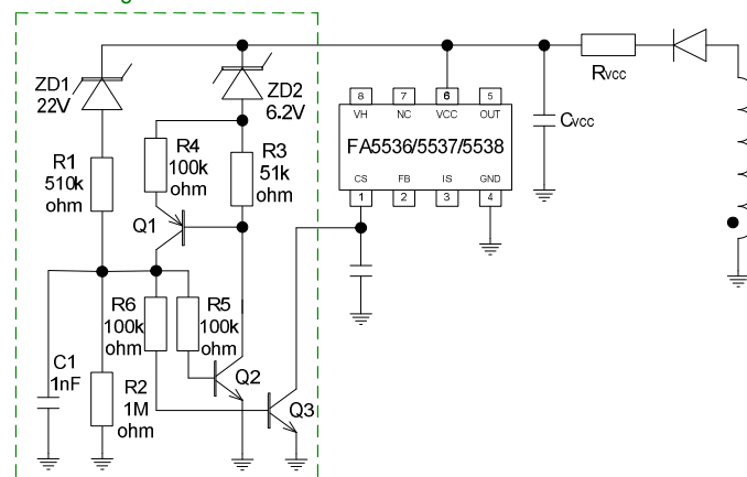
Fig.32 Over Voltage protection (1) for FA5536/37/38
