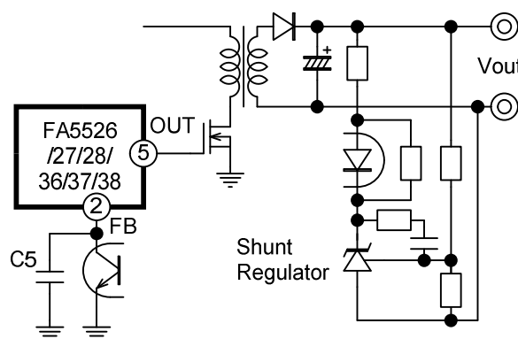
Fig.37 Prevention of malfunction caused by noise (FB pin)
