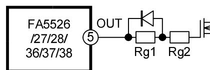
Fig.41 Gate circuit (1)
