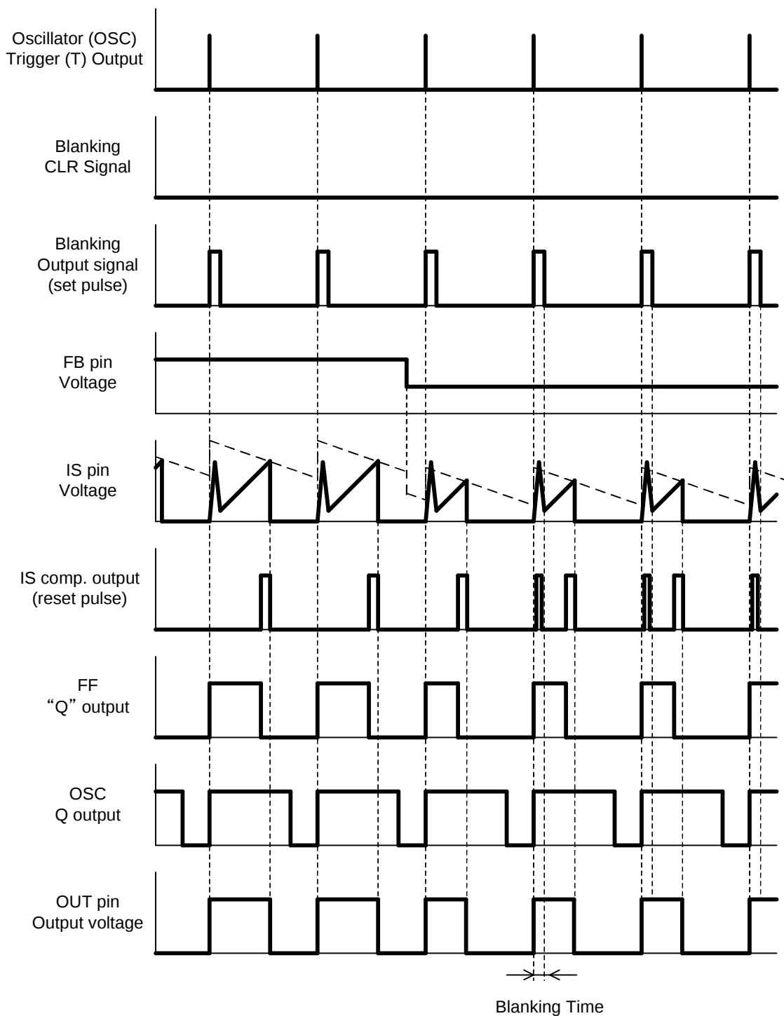
Fig.18 Timing chart at steady operation
