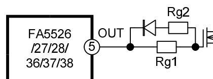
Fig.42 Gate circuit (2)
