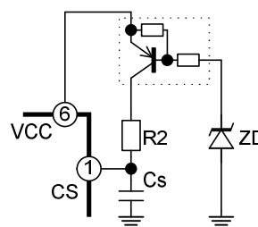
Fig.31 Over Voltage protection (3) for FA5526/27/28
